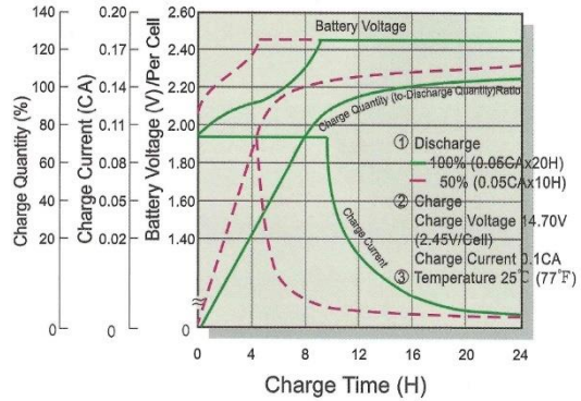
Cycle Charge
