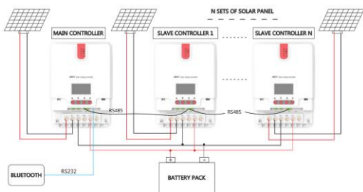
Parallel Controller Operation
